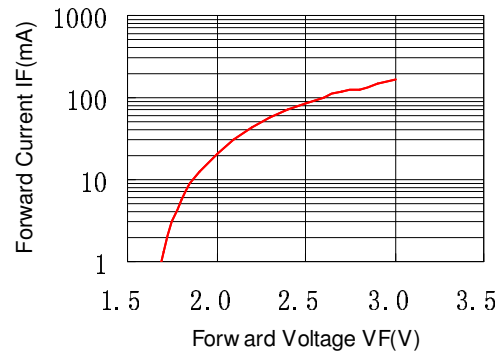
Forward Voltage vs. Forward Current (Ta=25°C)
