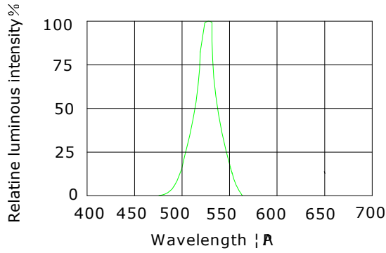
Spectrum Distribution Ta=25°
