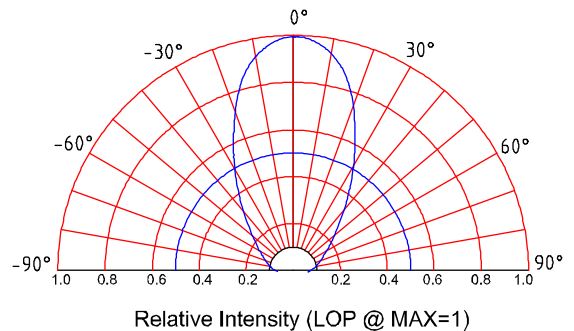
Beam Pattern
