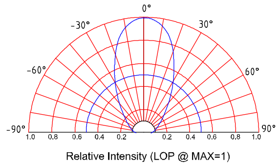
Beam Pattern
