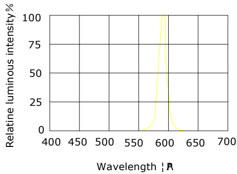
Spectrum Distribution Ta=25°
