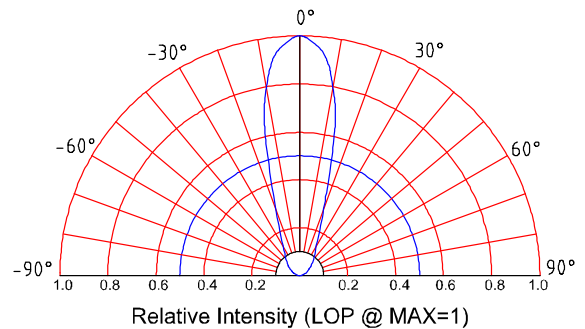
Beam Pattern
