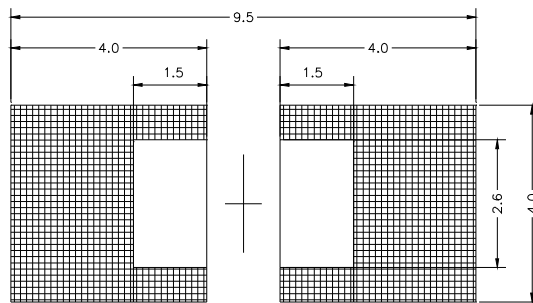
: Solder resist (Unit :mm)
