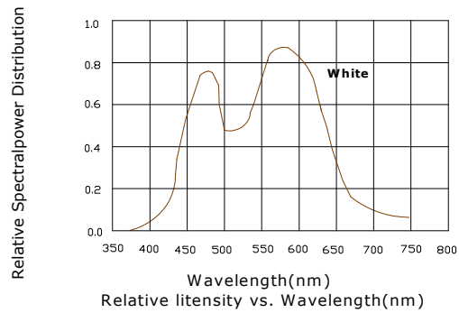
Spectrum Distribution on Ta=25°
